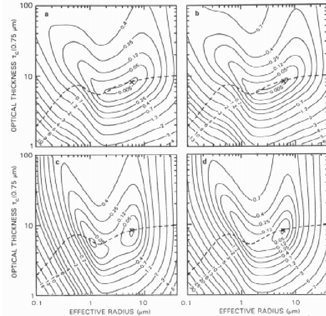
Figure 14. \chi^2 hypersurface for theoretically generated spherical albedo measurements at (a) 0.75 and 2.16 \mu\text{m} , (b) 0.75, 1.65 and 2.16 \mu\text{m} , (c) 0.75 and 3.70 \mu\text{m} , and (d) 0.75, 1.65, 2.16 and 3.70 \mu\text{m} . The solid curves represent constant values of \chi^2 , while the dashed curve in each panel represents the array of possible solutions for R_{\text{meas}}^{\text{vis}} = 0.495 . These results were constructed for a model cloud layer having \tau_c(0.75 \mu\text{m}) = 8 and r_e = 6 \mu\text{m} , located by the minimum value of \chi^2 in this two-dimensional space [from Nakajima and King (1990)].
