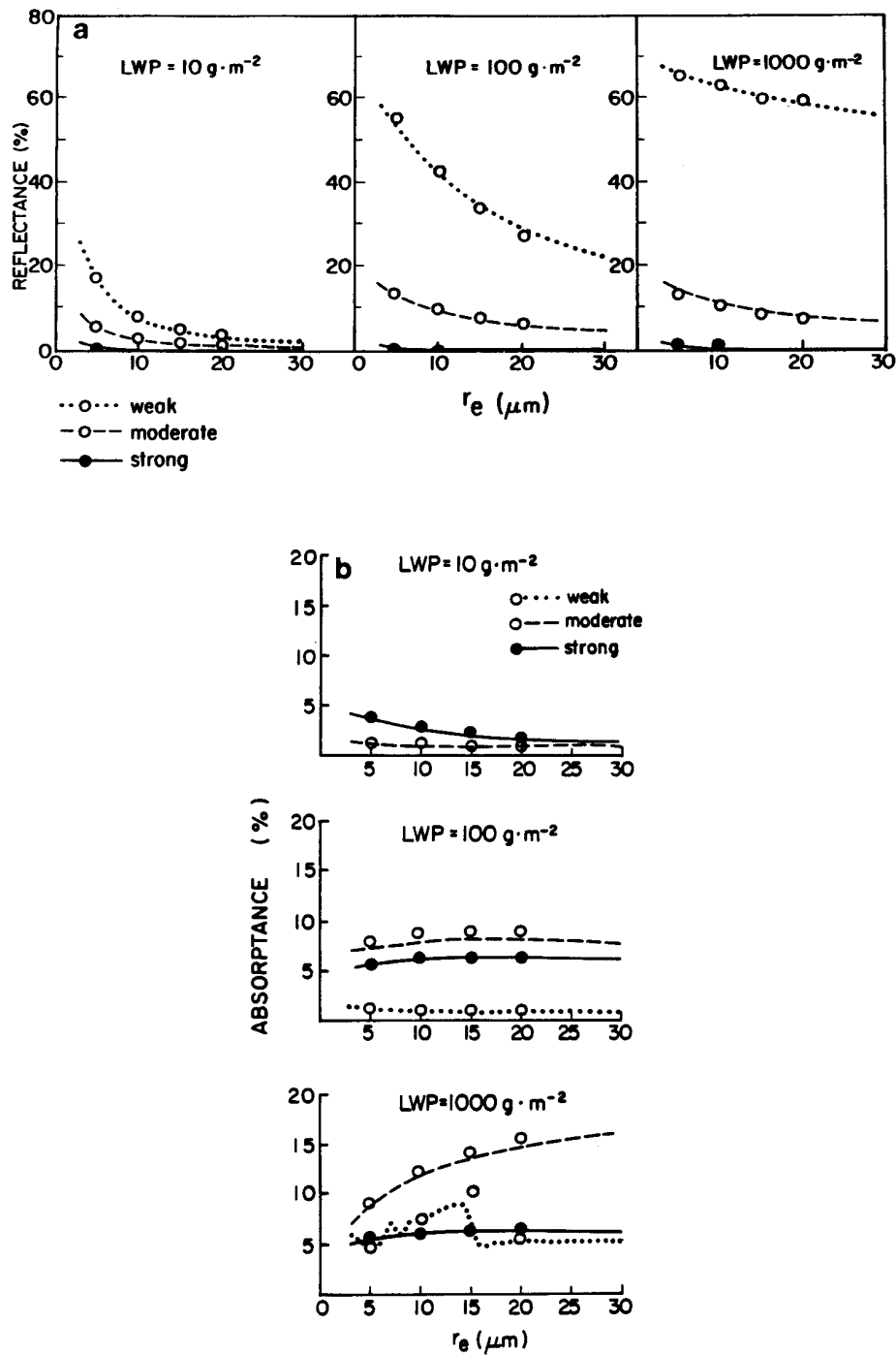
Figure 15. Contributions to (a) reflectance and (b) absorptance by the three absorption regimes as a function of r_e for cloud liquid water paths specified. The symbols refer to calculations performed using single-scattering properties determined from Mie theory (no significance should be attached to the difference between symbols) and the curves apply to calculations using the diffraction approximation to particle scattering assuming an overhead sun (after Ackerman and Stephens 1987).
