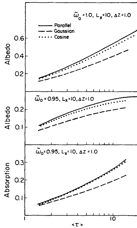
Figure 21. Albedo and absorptance as a function of area-averaged optical thickness, \langle \tau \rangle , for the plane parallel, cosine and Gaussian cloud distribution for the values of single-scatter albedo, horizontal scale of variability ( L_x ) and layer thickness \Delta z given (after Stephens 1988a).
