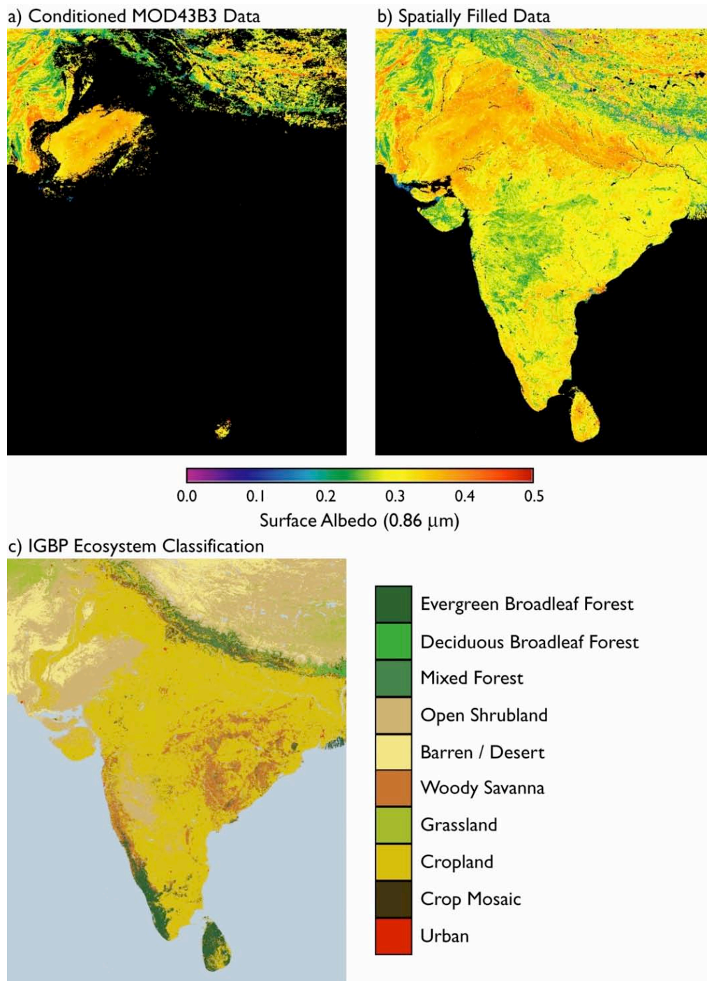
Fig. 7. Comparison of white-sky albedo at 0.86 \mu\text{m} for the Indian subcontinent for the June 10–June 26, 2002 sixteen-day time period, where (a) is the conditioned MOD43B3 data, (b) the spatially complete data, and (c) the IGBP ecosystem classification map used during processing.
