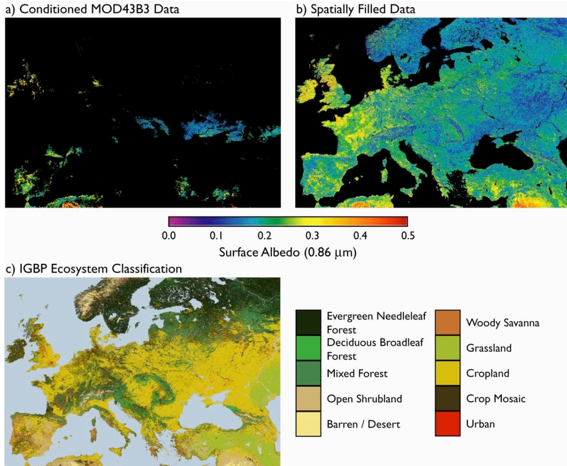
Fig. 6. Comparison of white-sky albedo at 0.86 \mu\text{m} for Europe and western Asia for the December 3-18, 2002 sixteen-day time period, where (a) is the conditioned MOD43B3 data, (b) the spatially complete data, and (c) the IGBP ecosystem classification map used during processing.
