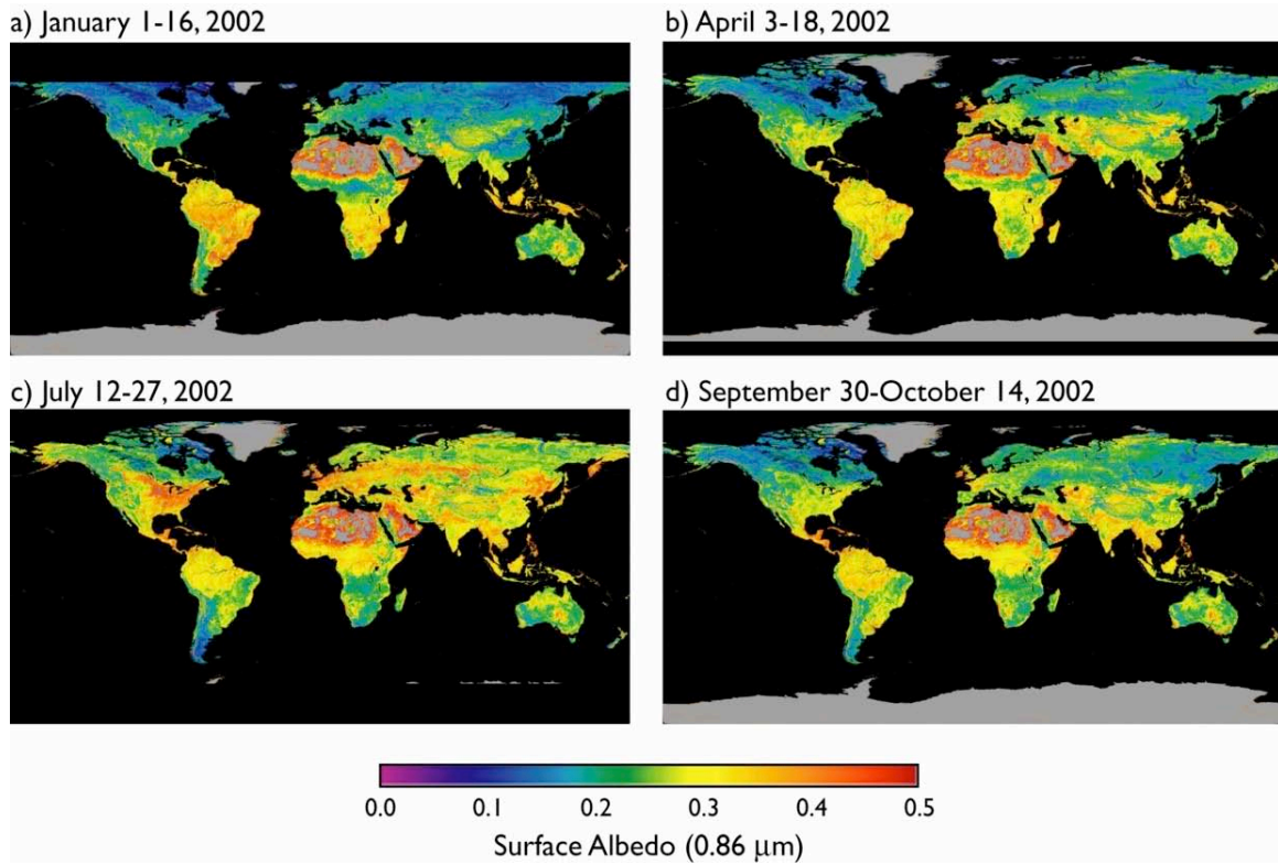
Fig. 10. Spatially complete white-sky albedo at 0.86 \mu\text{m} after the temporal interpolation technique was applied for the 16-day periods of (a) January 1-16, (b) April 3-18, (c) July 12-27, and (d) September 30-October 14, 2002.
