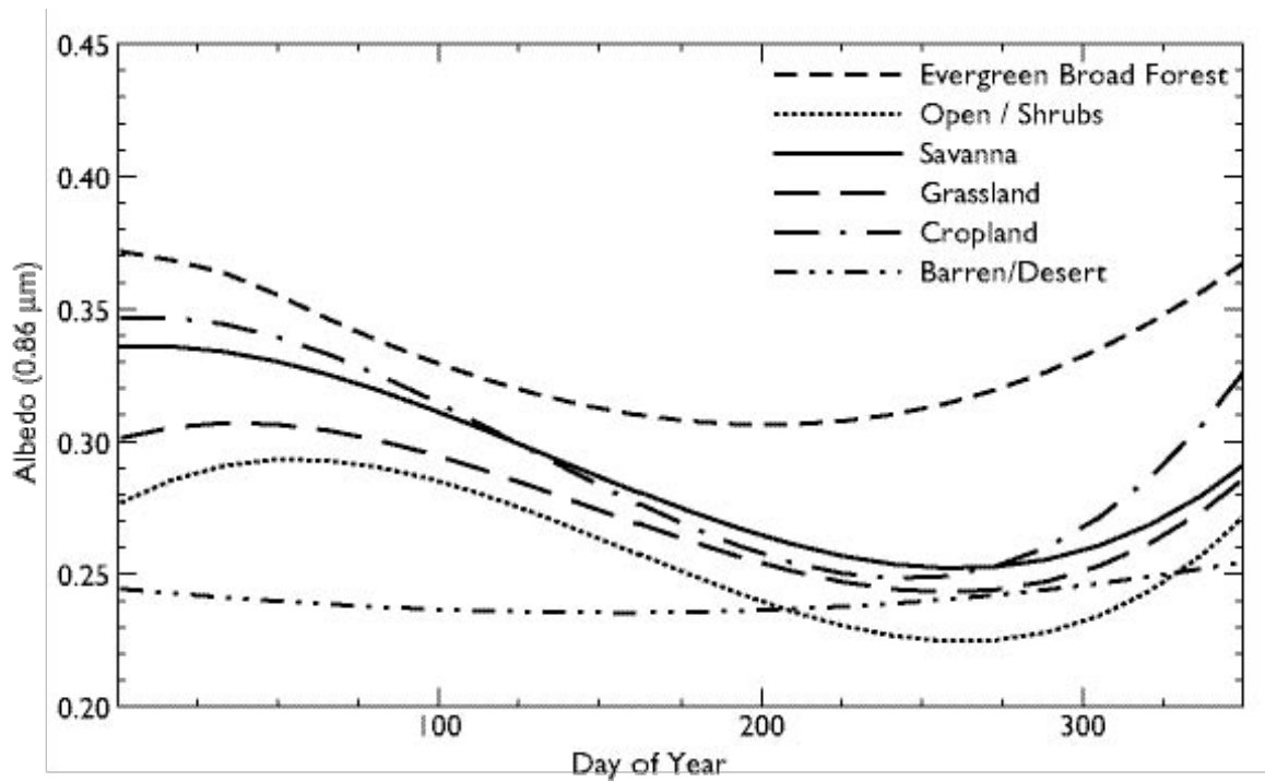
Fig. 9. 2002 Yearly trends for a selection of IGBP ecosystem classifications in the Amazon basin. The statistics are computed from the MOD43B3 data set using the South American latitude belt centered around 10 degrees south latitude.
