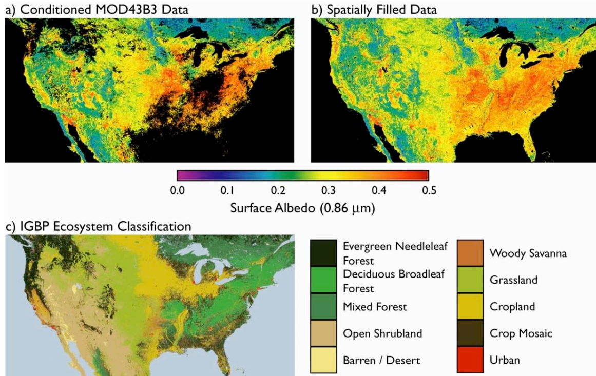
Fig. 4. Comparison of white-sky albedo at 0.86 \mu\text{m} for the continental United States for the July 12-27, 2002 sixteen-day time period, where (a) is the conditioned MOD43B3 data, (b) the spatially complete data, and (c) the IGBP ecosystem classification map used during processing.
