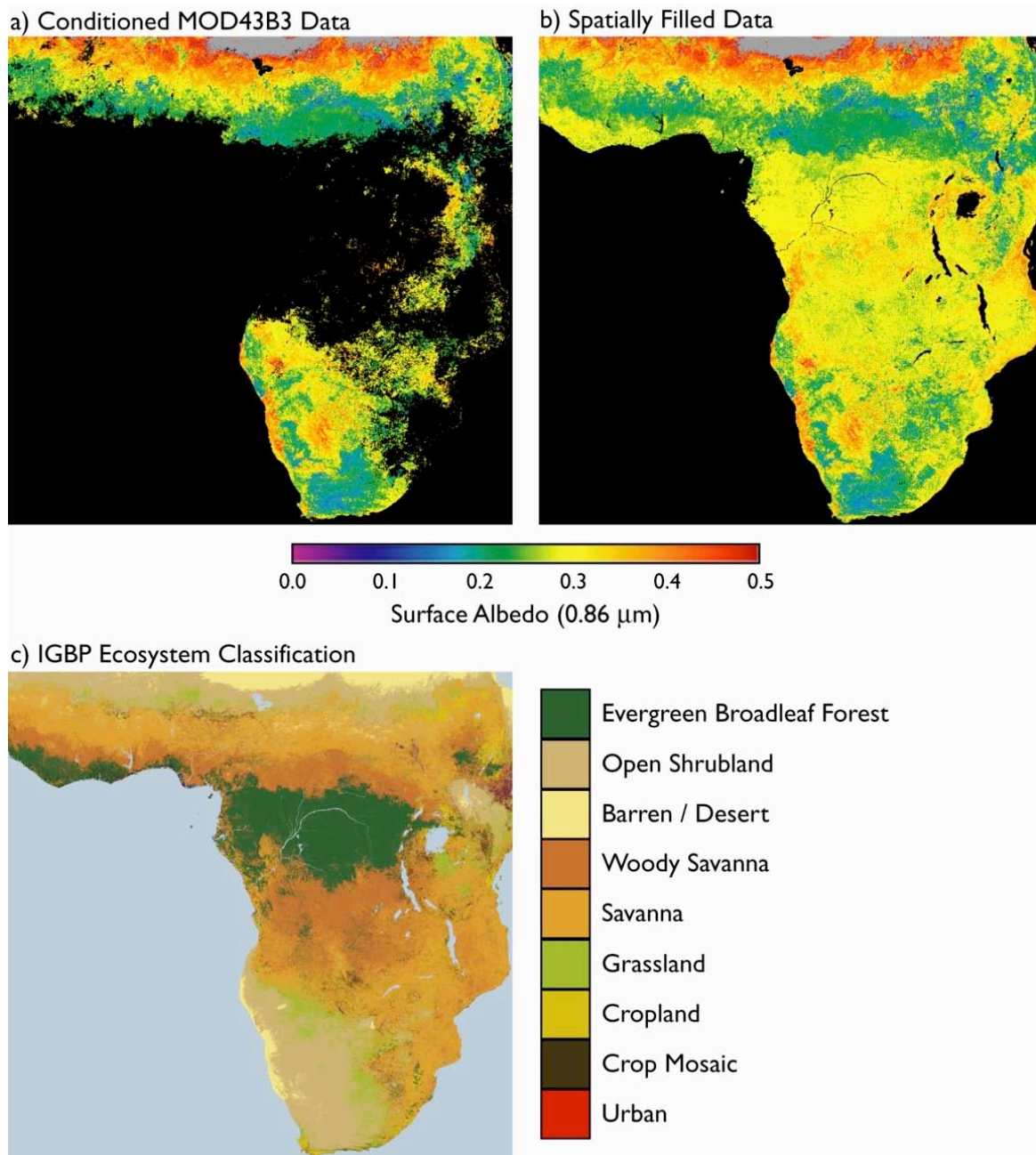
Fig. 8. Comparison of white-sky albedo at 0.86 \mu\text{m} for central and southern Africa, for the December 3-18, 2002 sixteen-day time period, where (a) is the conditioned MOD43B3 data, (b) the spatially complete data, and (c) the IGBP ecosystem classification map used during processing.
