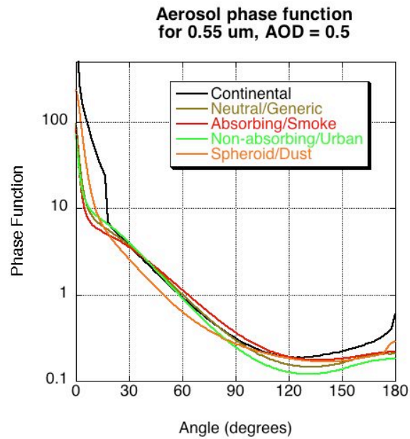
Figure 12: Plot of phase function at 0.55 \mu m (as a function of angle) for the 5 aerosol models in of the V5.2 LUT. In each case, \tau = 0.5 .
